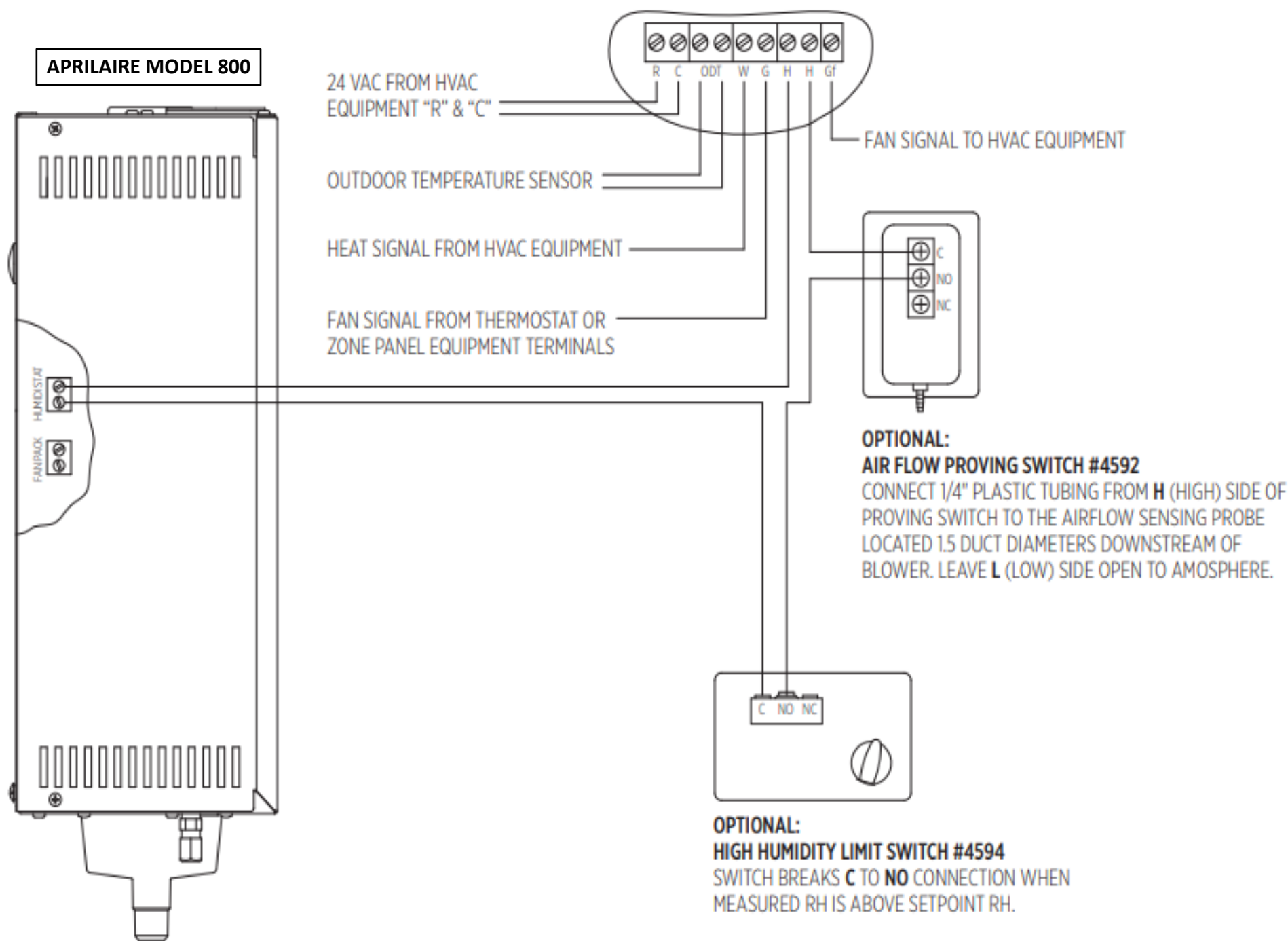
FIGURE 13- STEAM HUMIDIFIER ACCESSORY WIRING
